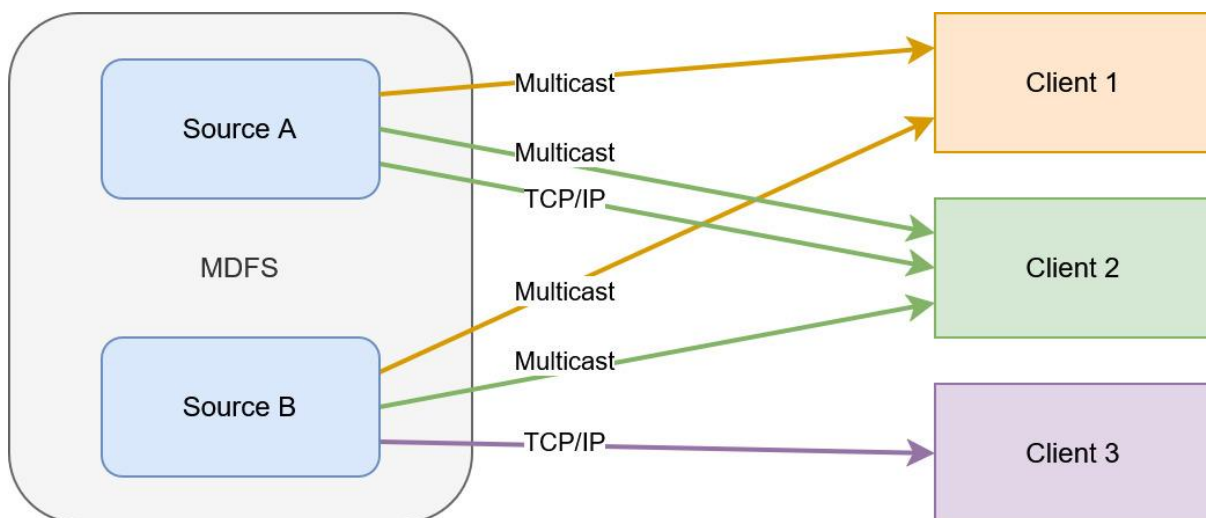
Figure 1 - Architecture Overview
